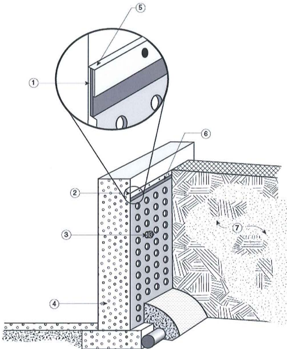
Figure 1. Installation details of “SUPERSEAL Dimpled Membrane (Dampproofing)” (front view)
