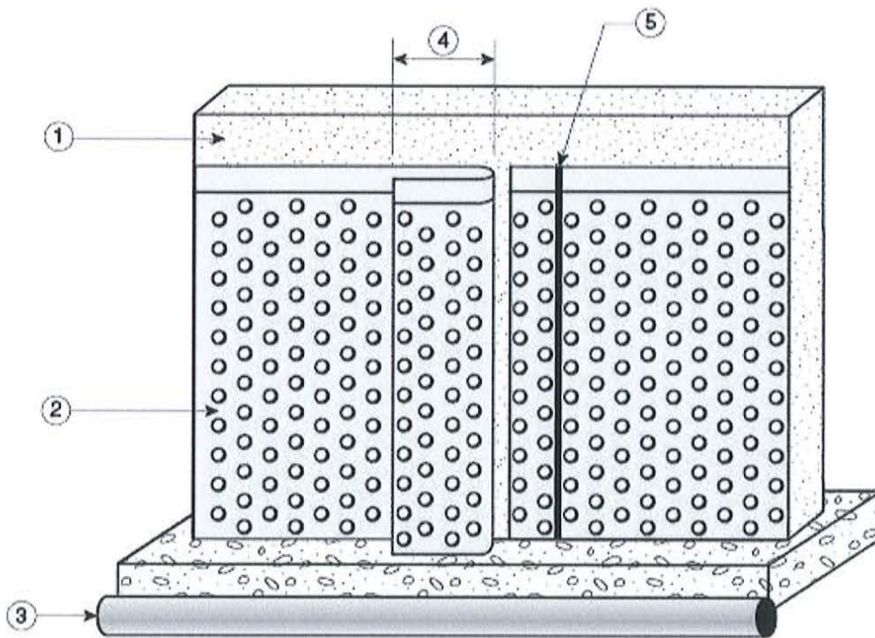
Figure 2. Installation details of "SUPERSEAL Dimpled Membrane (Dampproofing)" (side view)
